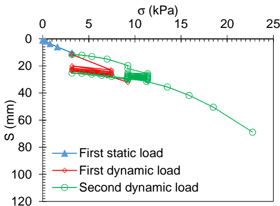
Figure 7: The relationship between S vs \sigma for reinforced peat under dynamic load
