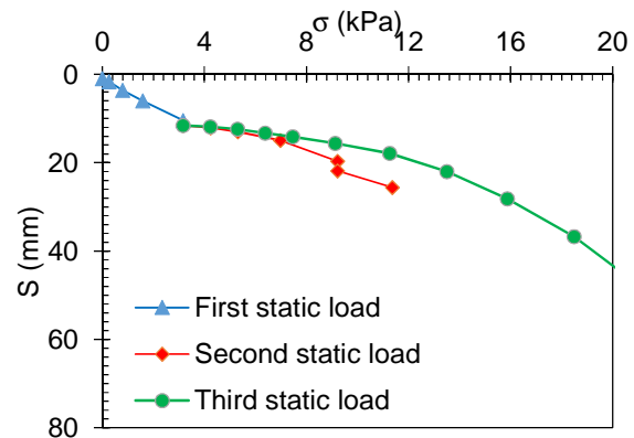
Figure 5: The relationship between S vs \sigma for reinforced peat under static load
