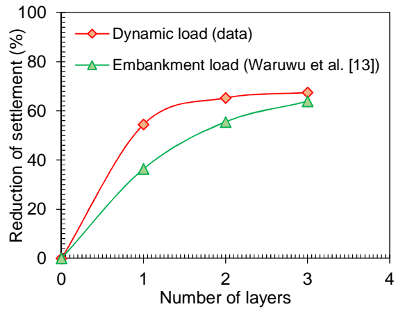
Figure 8: Result comparison of reduction of settlement for dynamic load and static load
