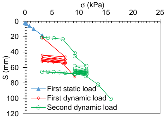
Figure 6: The relationship between S vs \sigma for unreinforced peat under dynamic load
