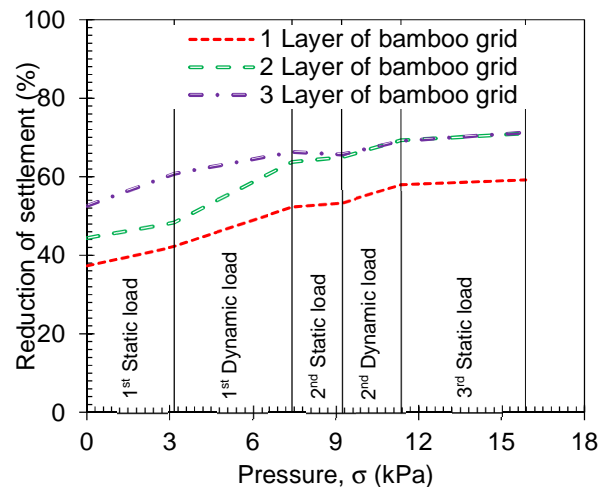
Figure 9: Effect of loading sequences on the reduction of settlement
