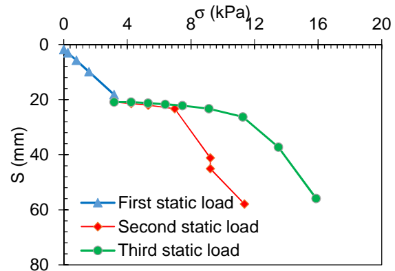
Figure 4: The relationship between S vs \sigma for unreinforced peat under static load
