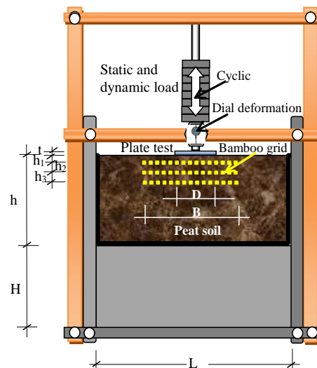
Figure 1: Model dimensions and bamboo grid configuration
