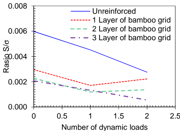
Figure 10: The relationship between ratio S/\sigma and number of dynamic loads
