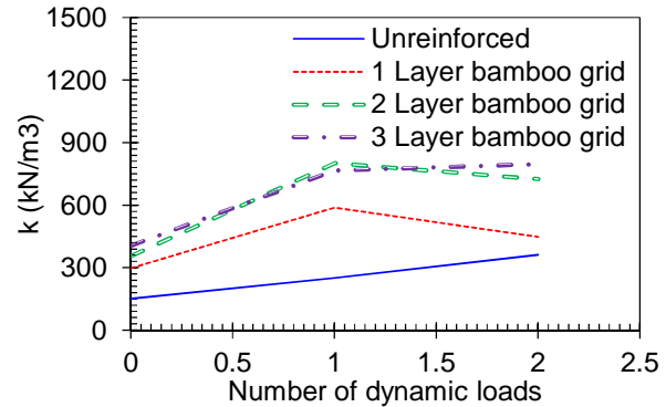
Figure 11: The relationship between modulus of subgrade reaction ( k ) and number of dynamic load
