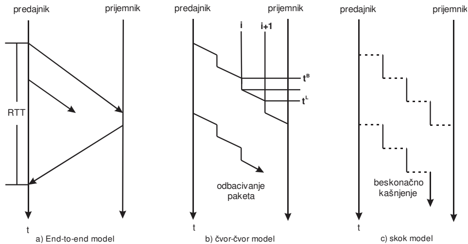
Slika 2. Prenos paketa Picture 2. Packet transmission
